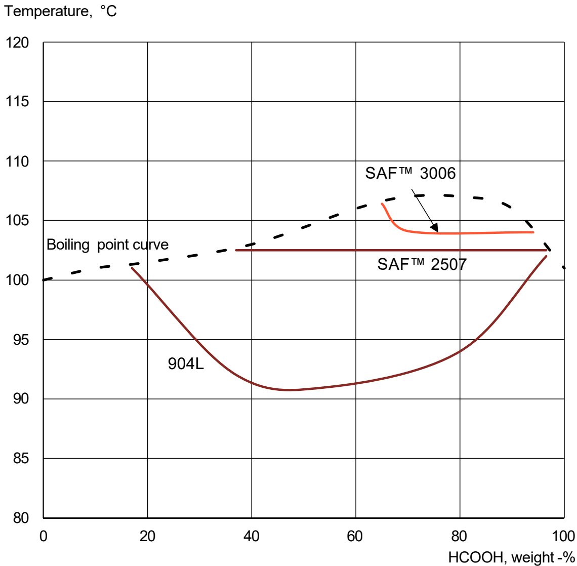
Figure 3 – Iso-corrosion in formic acid. The curves represent a corrosion rate of 0.1 mm/year (4 mpy) in stagnant test solution.
