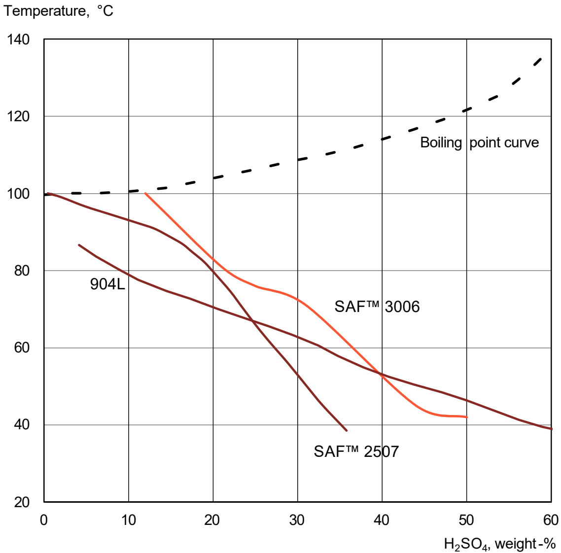
Figure 2 - Iso-corrosion in naturally aerated sulfuric acid. The curves represent a corrosion rate of 0.1 mm/year (4 mpy) in stagnant test solution.
