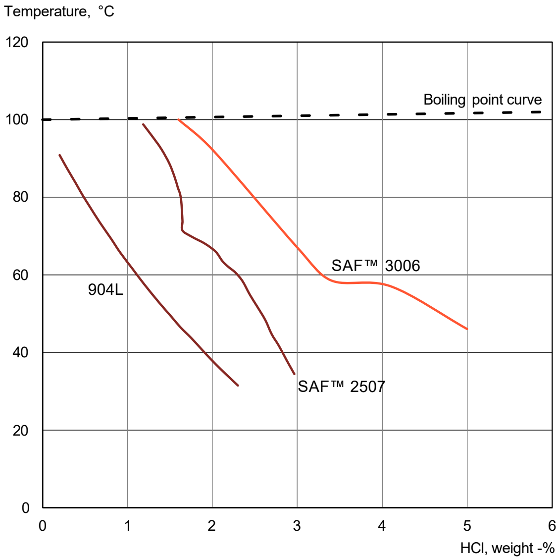
Figure 1 – Iso-corrosion in hydrochloric acid. The curves represent a corrosion rate of 0.1 mm/year (4 mpy) in stagnant test solution.
